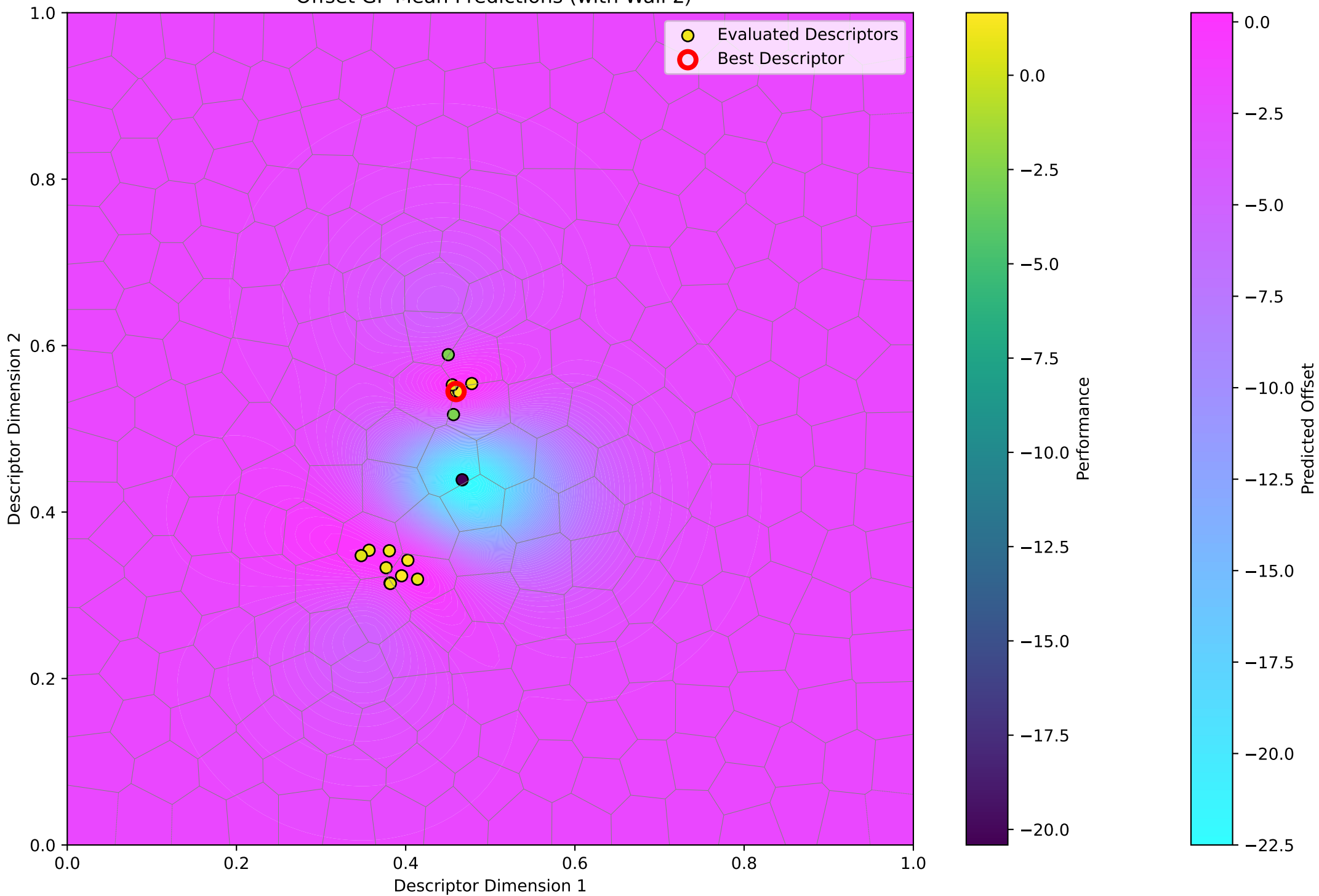
Offset GP Mean Predictions (with Wall 2)
