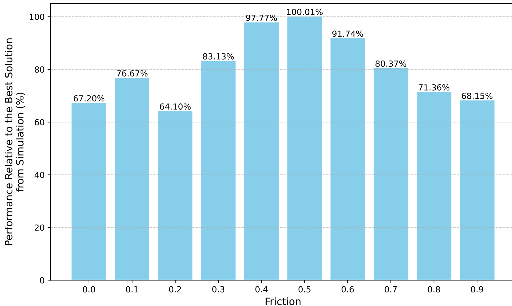
Performance of Found Solutions Across Different Friction Environments Relative to Best Solution from Simulation
