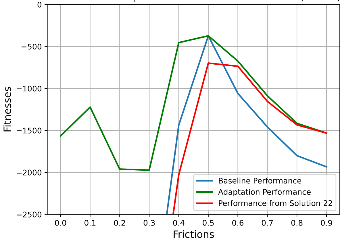
Baseline and Adaptation Performances vs. Friction (Scaled)
