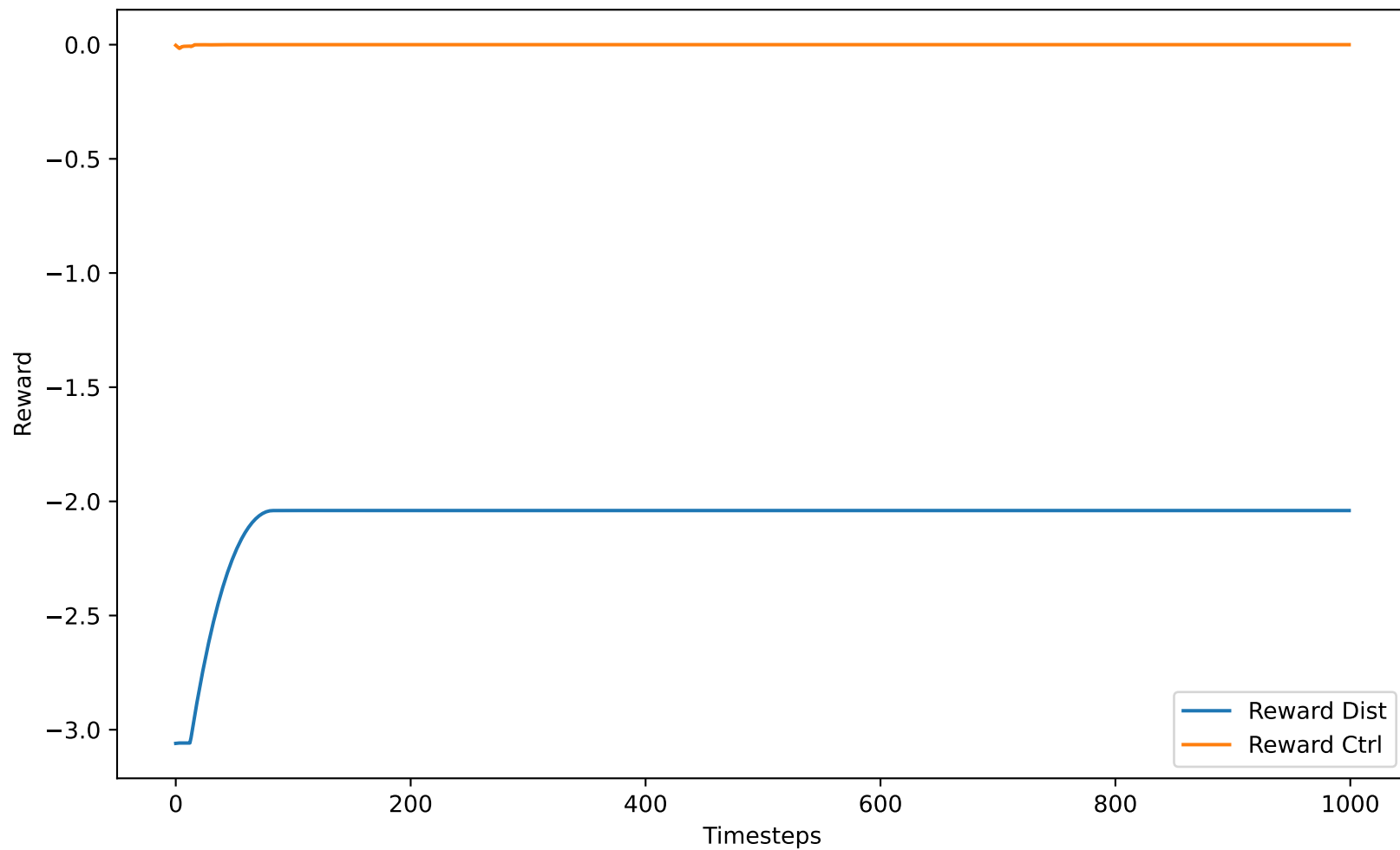
Reward Metrics Over Time
