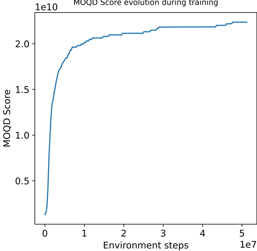
MOQD Score evolution during training
