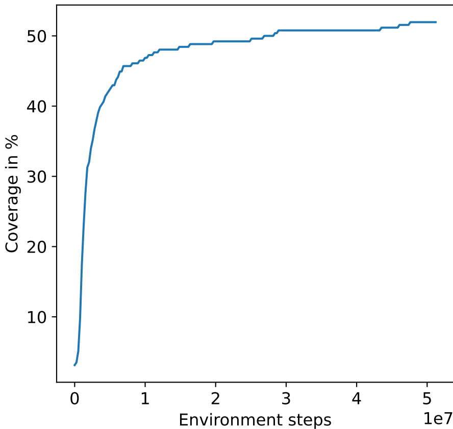
Coverage evolution during training
