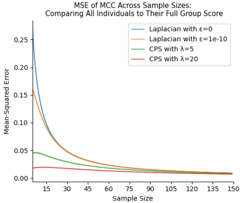
Figure 5.4: Comparison of smoothing techniques on metrics with undefined values. Bashful smoothing ( \epsilon = 1e^{-10} ) reduces errors compared to no smoothing ( \epsilon = 0 ). Cross-Prior Smoothing (CPS) offers further improvements, with the stronger prior ( \lambda = 20 ) outperforming the weaker prior ( \lambda = 5 ), indicating that CPS uses sufficiently informative priors.
