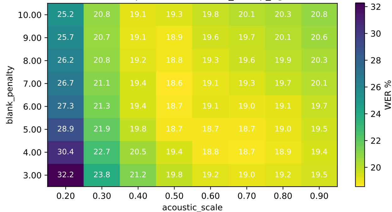
WER % heatmap — variant E (wer_sweep_5gram.csv)
