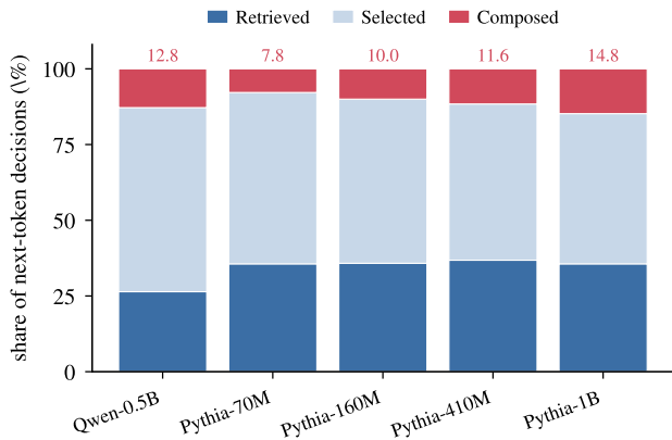
Figure 1: The same route split, visualised. Retrieval (RETRIEVED+SELECTED) dominates every model; the COMPOSED band (the irreducible computation, red, value annotated) grows monotonically up the Pythia ladder against a fixed store (7.8→14.8%), even as the geometry and margin structure stay scale-stable (Section 4).
