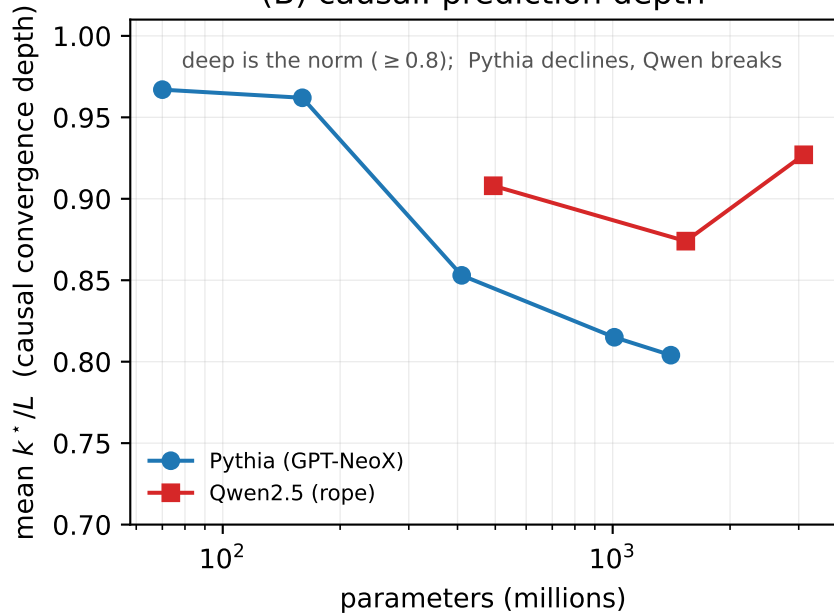
(B) causal: prediction depth
