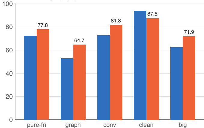
best-of-k deploy (%)
