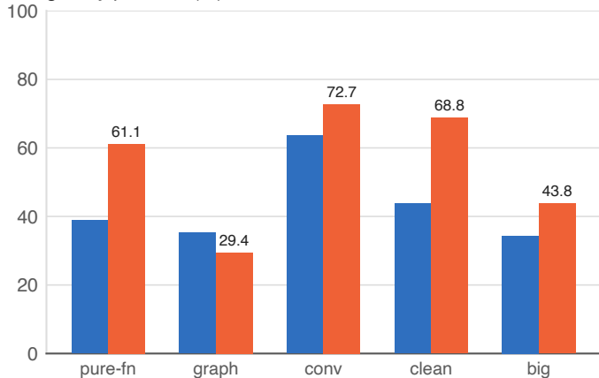
greedy pass@1 (%)
