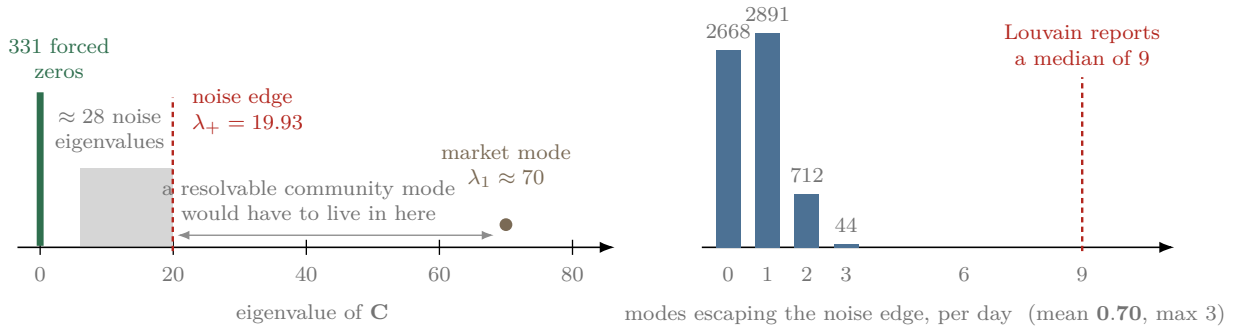
Figure 5: Left: where the eigenvalues of one day’s correlation matrix actually sit. Right: how many of them clear the noise edge, counted over all 6,315 days, against the number of communities Louvain reports. There is on average less than one statistically resolvable group per day beyond the market itself, and none at all on 2,668 days.
