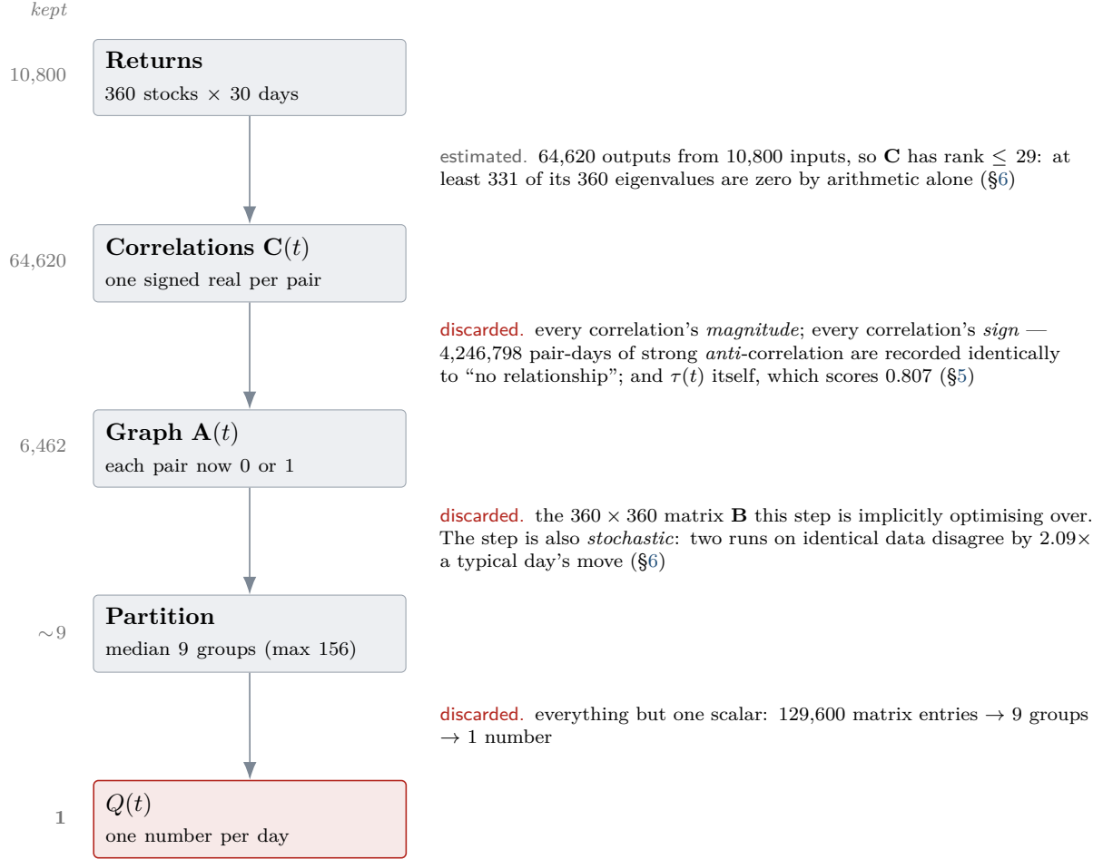
Figure 1: Silva’s pipeline as a sequence of reductions; the right-hand column is what each arrow costs. The paper reports the bottom box. The exploration in this document consists entirely of asking what is in the boxes above it, and scoring those contents on the paper’s own ruler.
