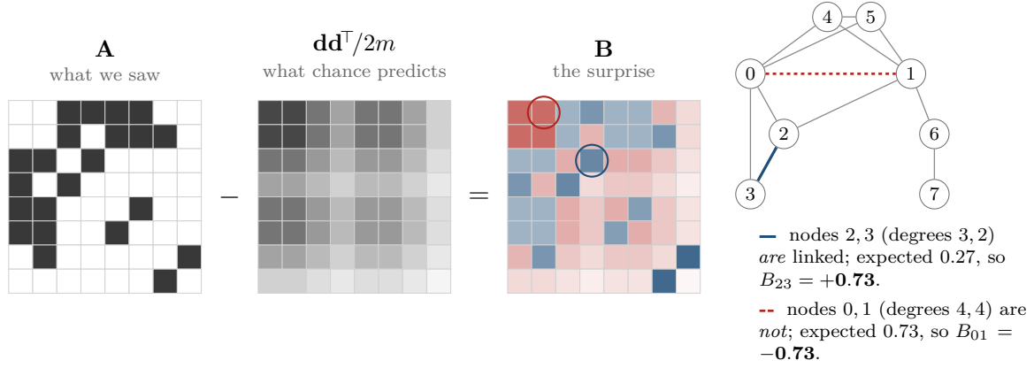
Figure 2: \mathbf{B} = \mathbf{A} - \mathbf{d}\mathbf{d}^\top/2m on an eight-node graph, drawn to scale; blue is positive surprise, red negative, intensity \propto |B_{ij}| . The two circled cells have identical magnitude and opposite sign — yet only one of them corresponds to an edge that exists. Subtracting the chance baseline turns a 0/1 matrix into a signed one, and what appears is exactly the information about pairs that are less connected than they should be. Every row of \mathbf{B} sums to zero.
