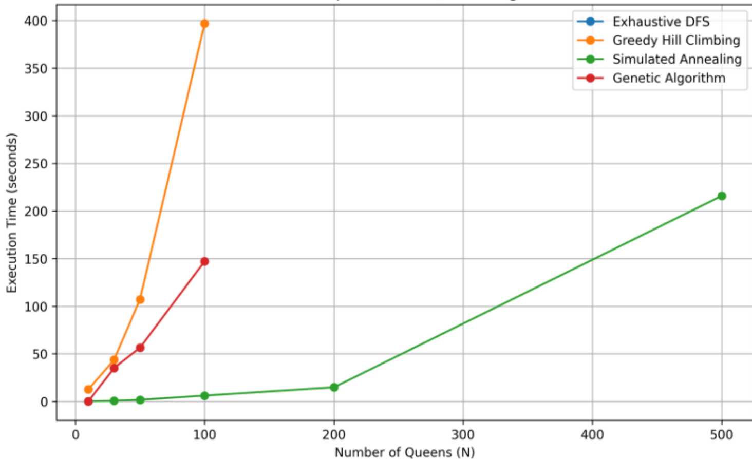
Runtime Comparison of N-Queens Algorithms
