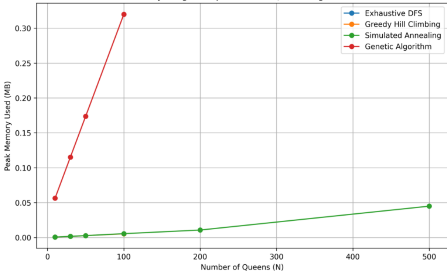
Memory Usage Comparison of N-Queens Algorithms
