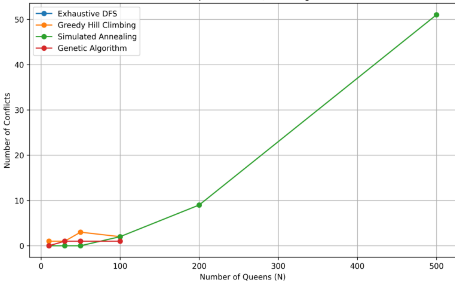
Conflict Comparison of N-Queens Algorithms
