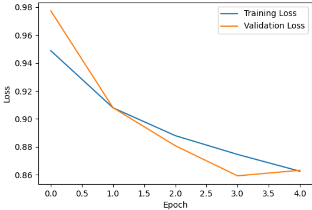
Custom CNN Loss Curve
