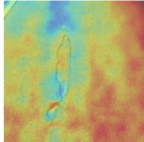
Pred: pothole (47.7%)
