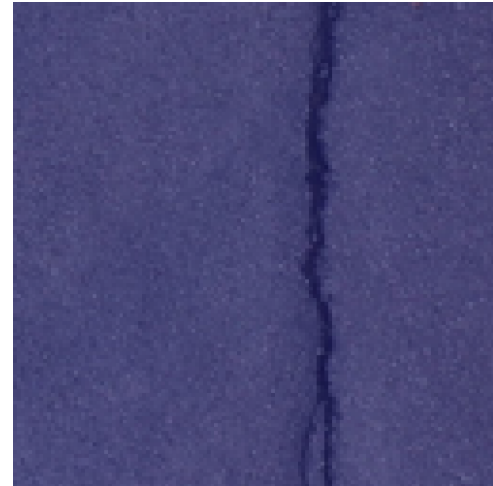
Pred: pothole (45.8%)
