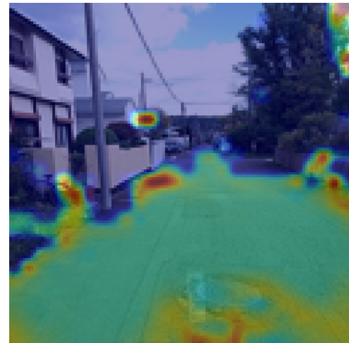
Pred: manhole (66.8%)
