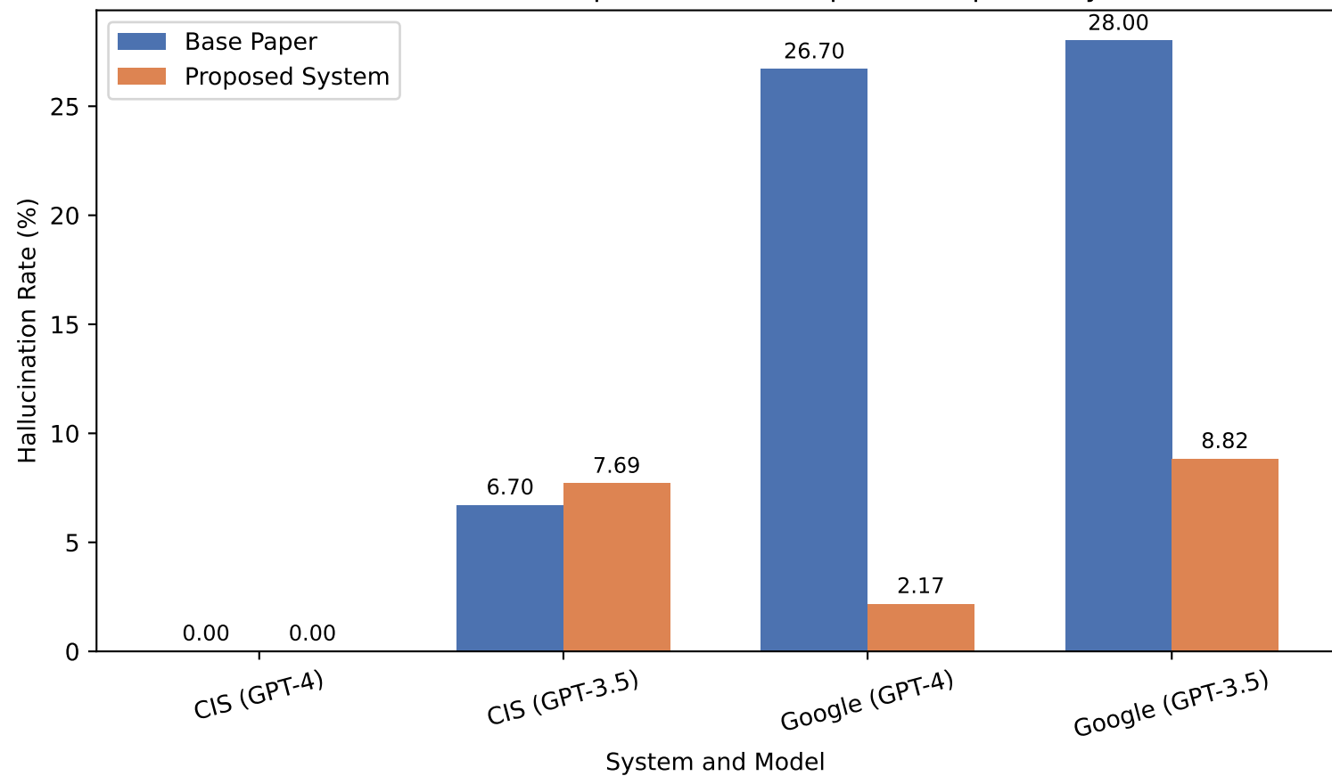
Hallucination Rate Comparison: Base Paper vs Proposed System
