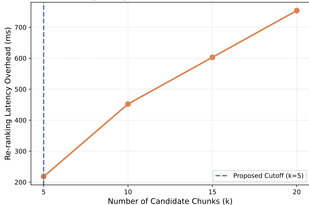
Ablation Study: Computational Overhead of Retrieved Chunks
