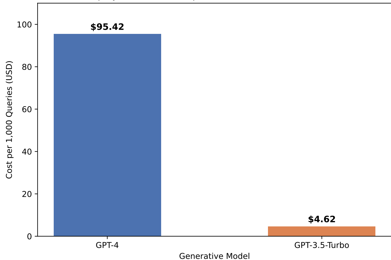
Deployment Cost Comparison: GPT-4 vs GPT-3.5-Turbo
