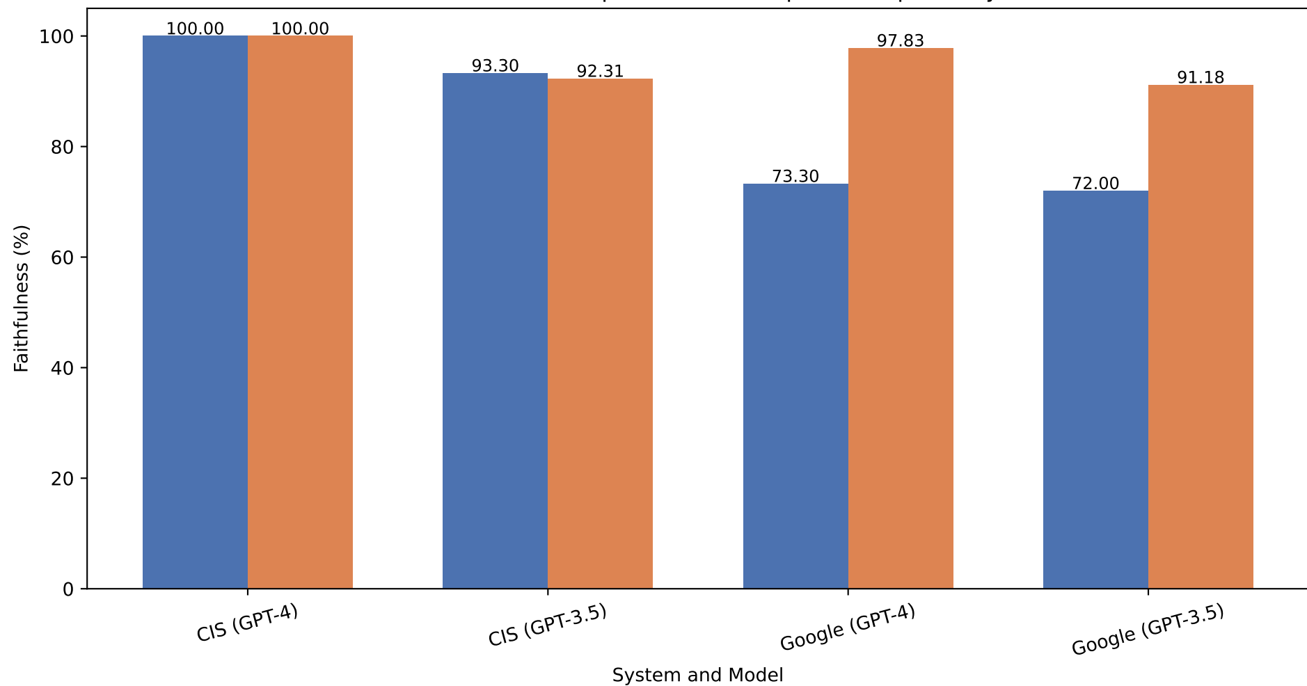
Faithfulness Score Comparison: Base Paper vs Proposed System
