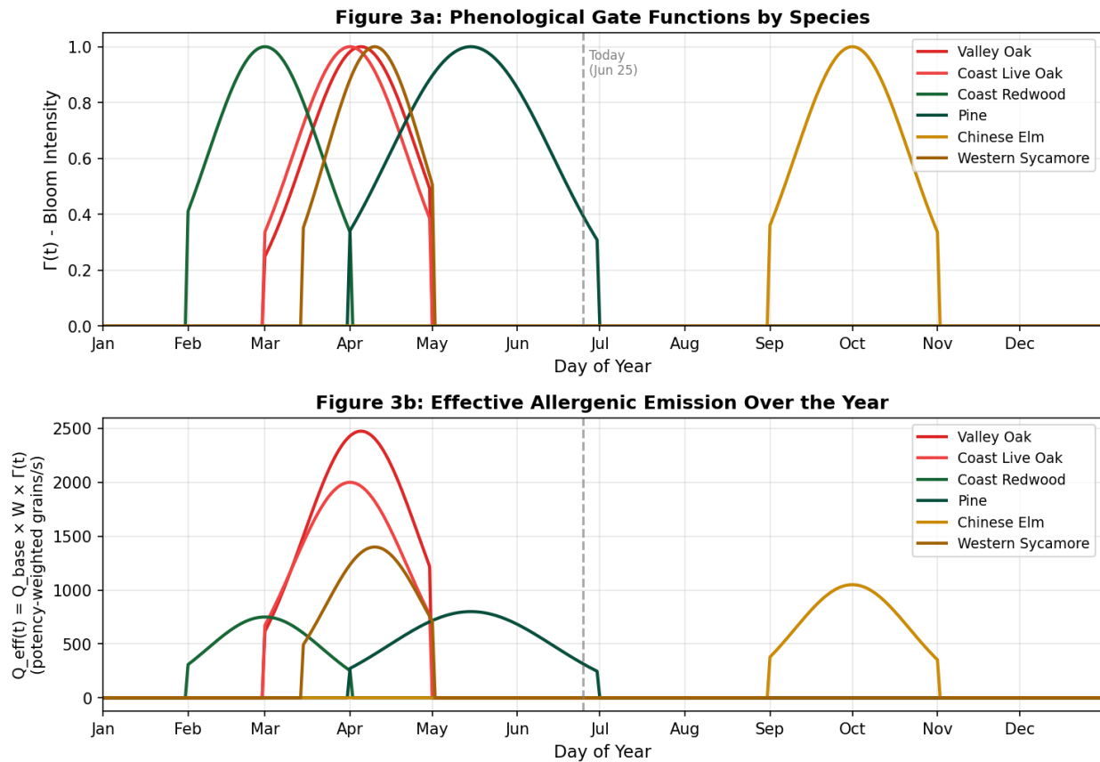
Figure 4: Phenological emission model. (a) Temporal gate functions \Gamma_i(t) showing blooming intensity across the year for each species. (b) Effective allergenic emission Q_{eff}(t) = Q_{base} \times W \times \Gamma(t) . The dashed line marks today (June 25), when most tree species are dormant and only Pine retains weak late-season emission.
