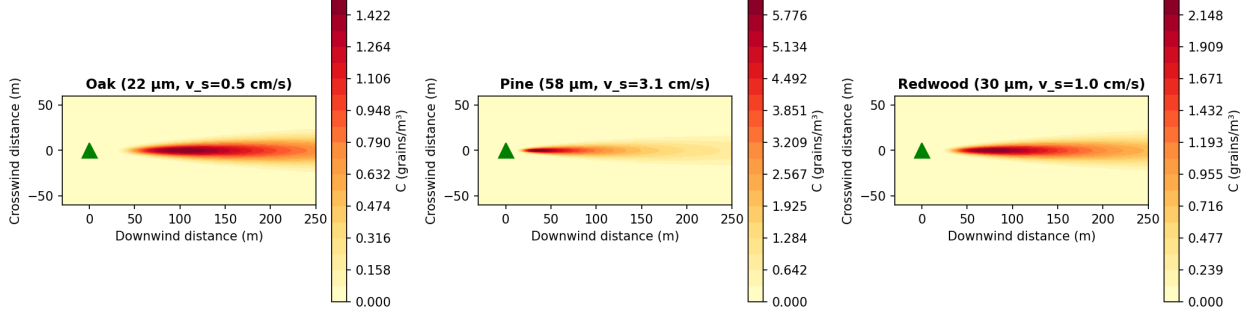
Figure 3: Species-dependent plume shapes due to different settling velocities. Oak pollen (small, light grains) produces wide, far-reaching plumes. Pine pollen (large, heavy grains) creates intense but localized concentration near the source tree.
