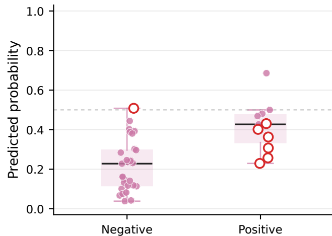
Random Forest
