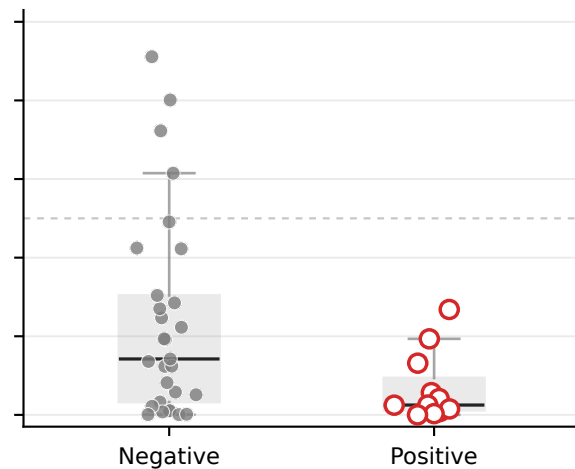
MLP-full features
