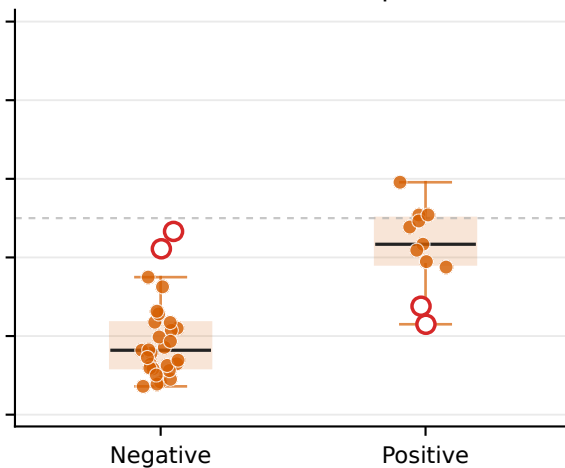
XGBoost
