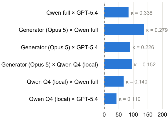
(b) Observed co-marks \div expected by chance
