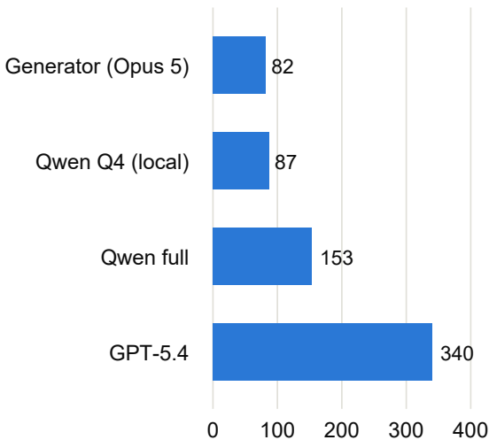
(a) Marked pairs per marker
