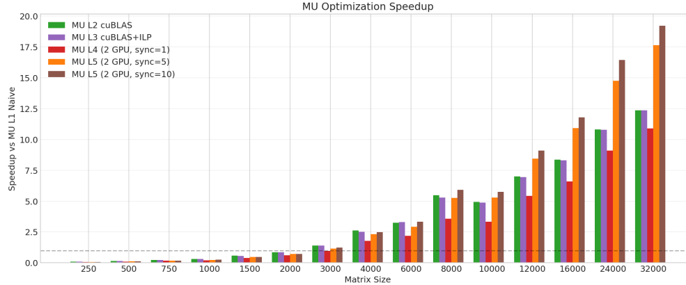
Figure 2: MU Speedup. Speedup relative to the naive L1 baseline. cuBLAS provides up to 12\times speedup on a single GPU, while async multi-GPU (L5 sync=10) achieves 19\times at size 32,000.
