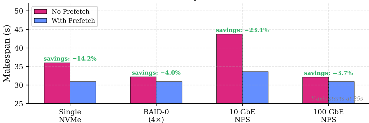
(b) End-to-End Makespan (60 tasks, 2 models)
