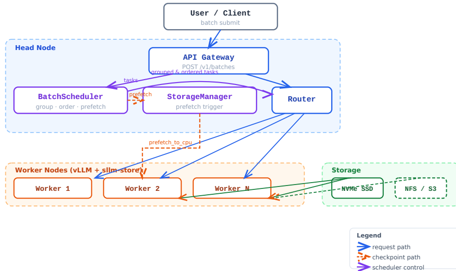
Figure 4.1: System architecture. The BatchScheduler on the head node groups tasks by model and applies Johnson’s Rule ordering. The StorageManager triggers asynchronous checkpoint prefetching to worker nodes. Workers run vLLM with slim-store for pinned memory management.
