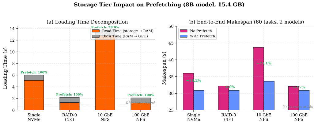
Figure 5.7: Storage tier impact on prefetching (8B model, 15.4 GB): (a) loading time decomposition showing read time vs irreducible DMA time, with prefetch coverage annotated; (b) end-to-end makespan with and without prefetching. Prefetching provides the largest benefit for 10 GbE NFS (23.1% reduction), where read latency is highest.
