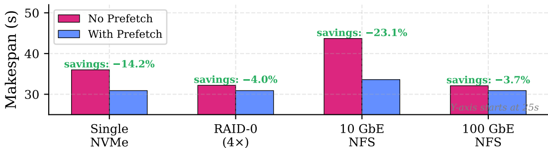
(b) End-to-End Makespan (60 tasks, 2 models)
