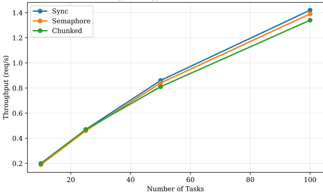
Scheduling Strategy Performance vs Task Count
