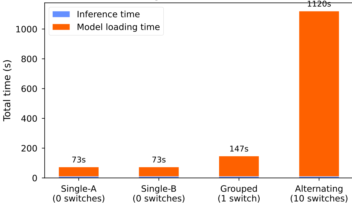
Model Switching Overhead (20 tasks, 2 models)
