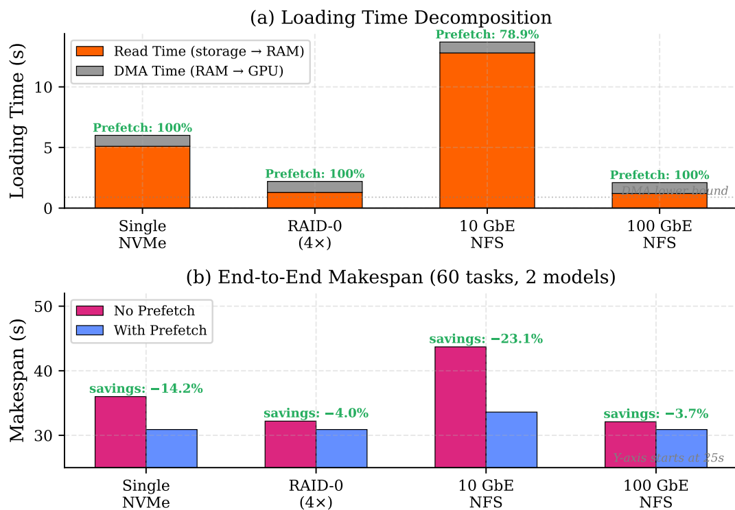
Figure 4.5: Storage tier impact on prefetching (8B model, 15.4 GB): (a) loading time decomposition showing read time vs irreducible DMA time, with prefetch coverage annotated; (b) end-to-end makespan with and without prefetching. Prefetching provides the largest benefit for 10 GbE NFS (23.1% reduction), where read latency is highest.
