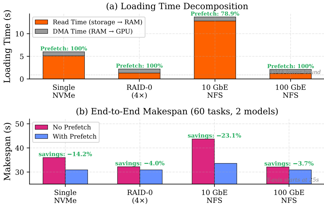
Figure 4.5: Storage tier impact on prefetching (8B model, 15.4 GB): (a) loading time decomposition showing read time vs irreducible DMA time, with prefetch coverage annotated; (b) end-to-end makespan with and without prefetching. Prefetching provides the largest benefit for 10 GbE NFS (23.1% reduction), where read latency is highest.
