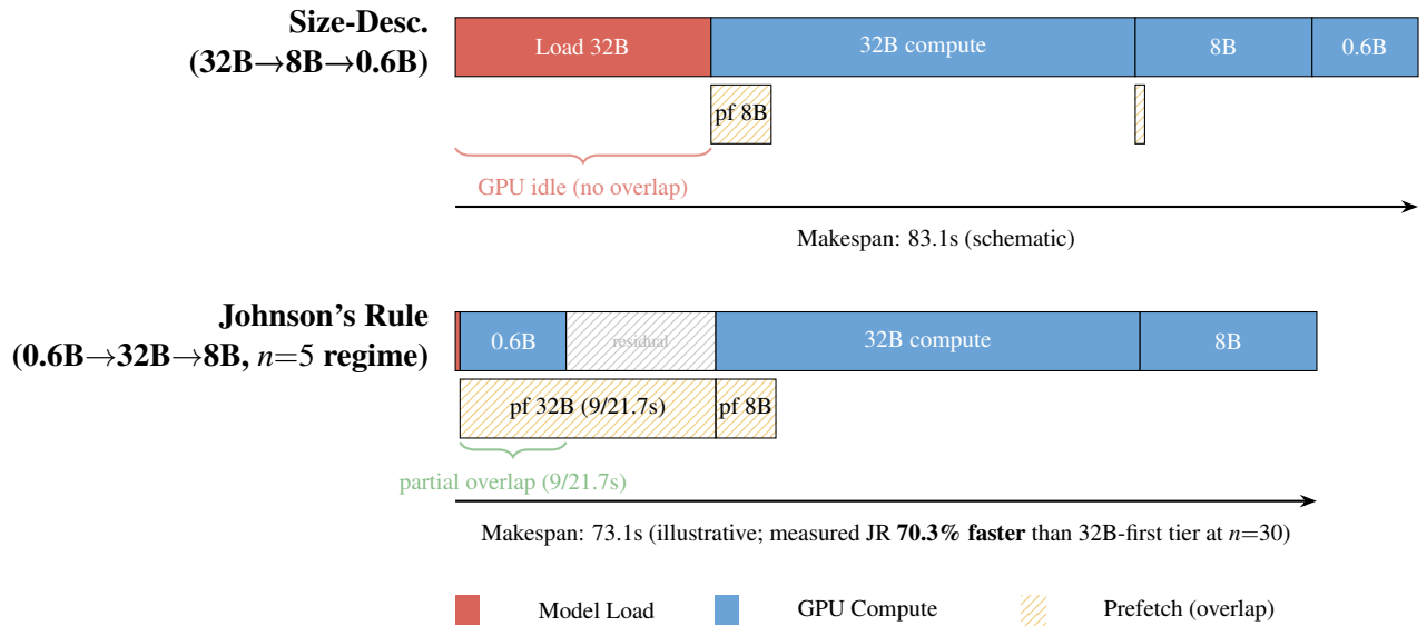
Figure 4.4: Schematic execution timeline: worst-case (32B-first, top) vs Johnson's Rule (0.6B-first, bottom) ordering. Placing the largest model first forces an unmasked GPU idle at t = 0 ; placing the smallest model first allows prefetching to begin immediately, reducing the residual gap.
