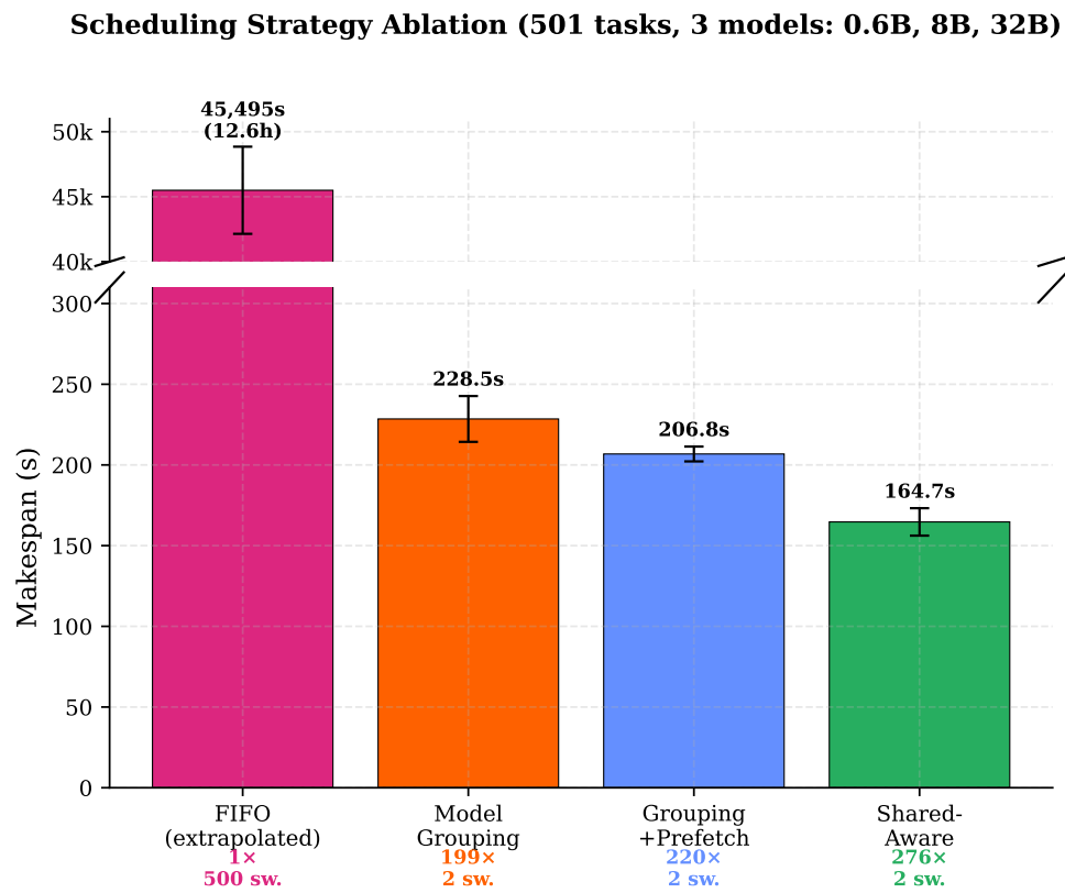
Figure 4.1: Incremental scheduling strategy ablation for 501 tasks with 3 models (0.6B, 8B, 32B). Each column adds one optimisation component.
