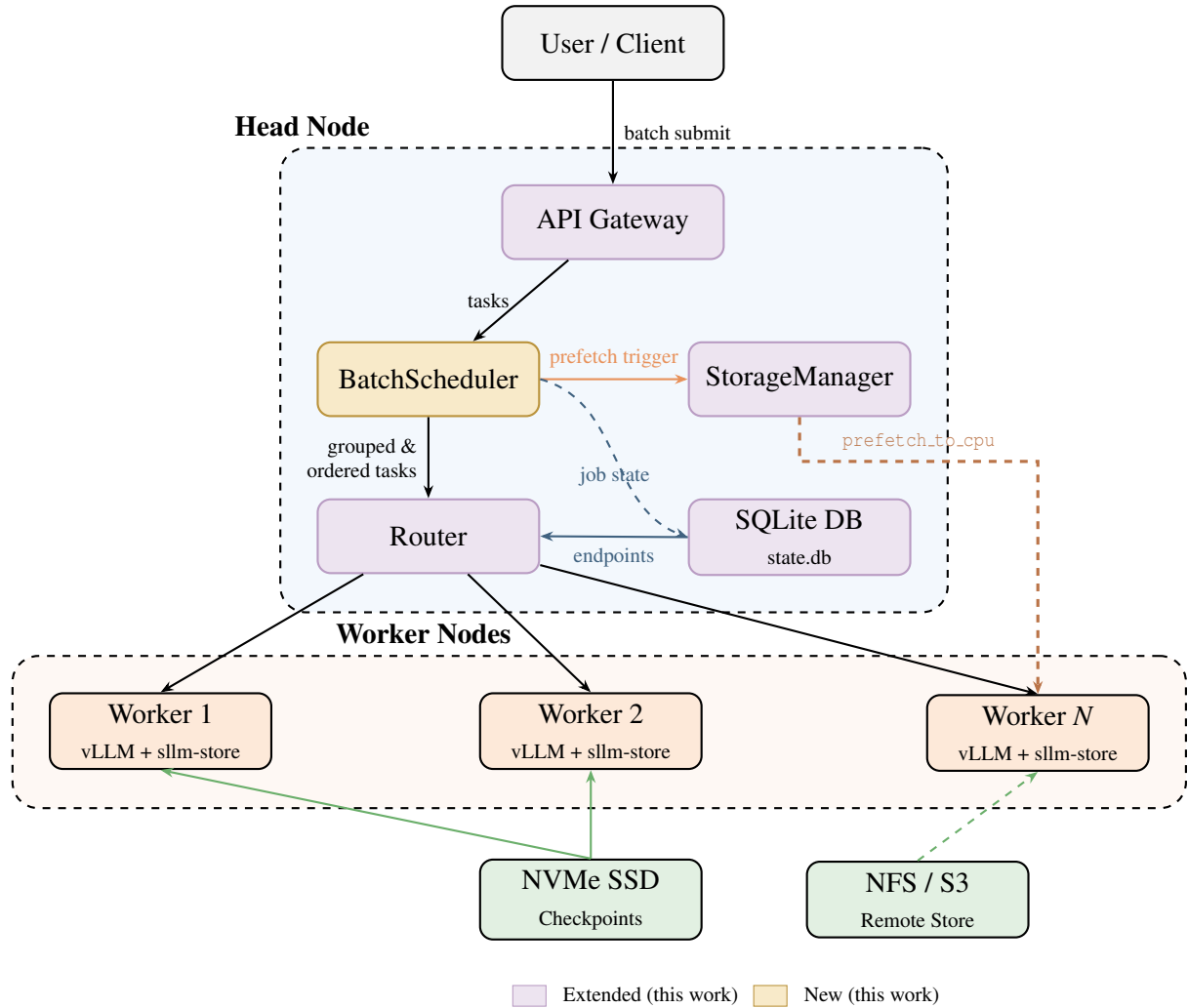
Figure 3.1: System architecture. The BatchScheduler groups tasks by model, applies Johnson’s Rule ordering, and persists job state to a SQLite database. The Router queries the same database for healthy worker endpoints. The StorageManager triggers asynchronous checkpoint prefetching ( prefetch_to_cpu ) to worker nodes ahead of execution. Workers run vLLM with sllm-store for pinned-memory checkpoint management.
