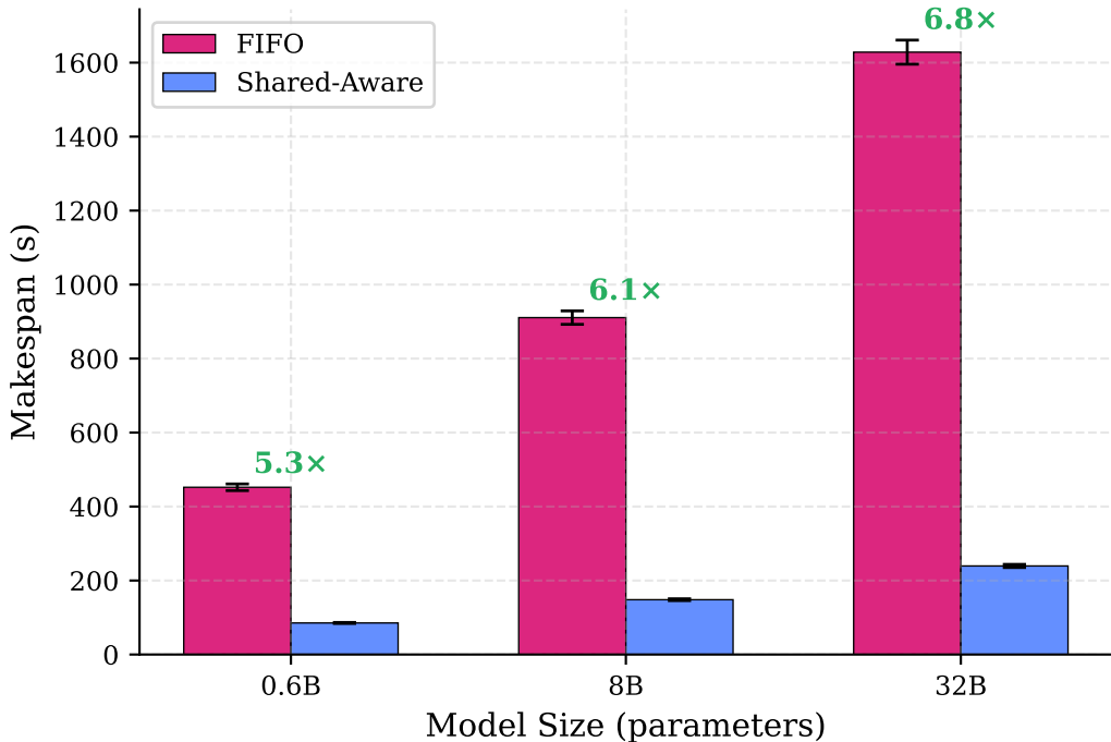
Robustness Across Model Sizes (50 tasks per model)
