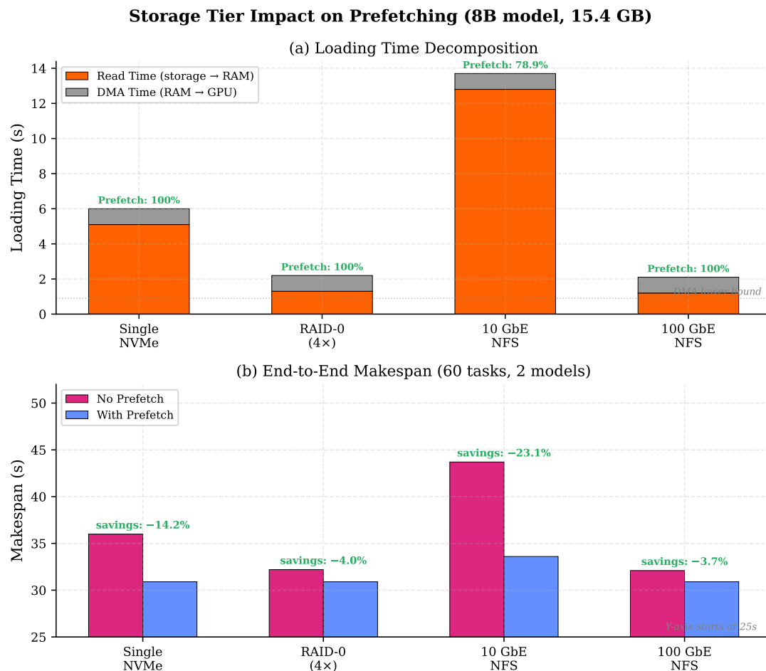
Figure 4.5: Storage tier impact on prefetching (8B model, 15.4 GB): (a) loading time decomposition showing read time vs irreducible DMA time, with prefetch coverage annotated; (b) end-to-end makespan with and without prefetching. Prefetching provides the largest benefit for 10 GbE NFS (23.1% reduction), where read latency is highest.
