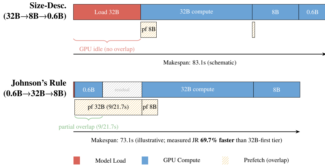
Figure 5.4: Execution timeline comparison (schematic): worst-case vs Johnson's Rule ordering for a 3-model batch. Worst case (top) places the I/O-heavy 32B model first, forcing 21.7s of unmasked GPU idle before any inference begins. Johnson's Rule (bottom) places the compute-heavy 0.6B group first to start the 32B prefetch early, then executes 32B while the trivially small 8B checkpoint loads, then finishes with 8B. The residual gap (12.7s) is smaller than the worst-case upfront idle (21.7s). In the measured experiment (Table 5.4), the worst-tier orderings (32B-first) averaged 225.5s vs 132.9s for JR (0.6B→32B→8B), a 69.7% difference; the spread across all six permutations is 94.9s.
