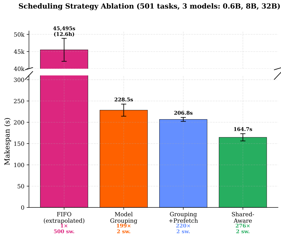
Figure 4.1: Incremental scheduling strategy ablation for 501 tasks with 3 models (0.6B, 8B, 32B). FIFO ( \approx 12.6\text{h} , computed from direct cold-start measurements) is shown on a separate axis. Each column adds one optimisation component.
