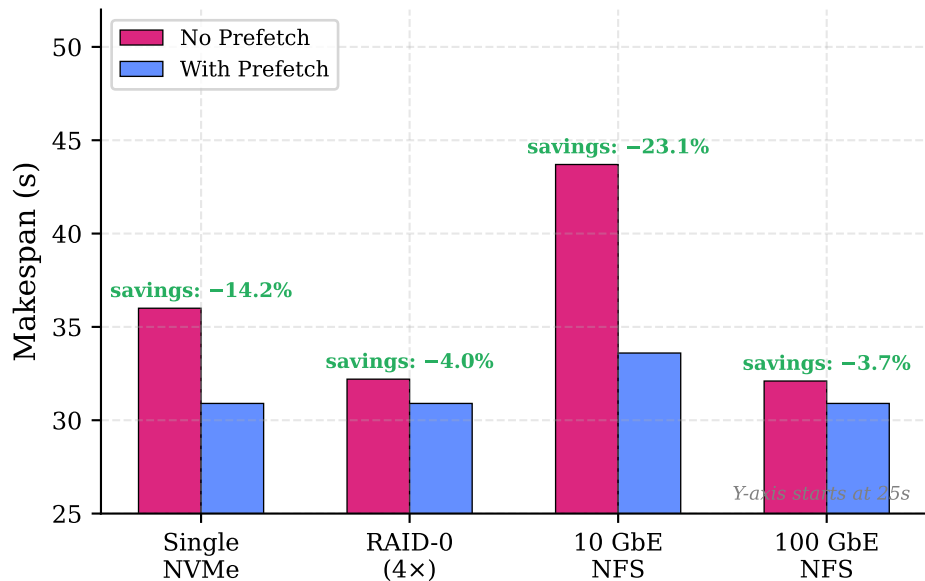
(b) End-to-End Makespan (60 tasks, 2 models)
