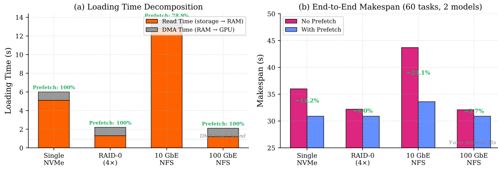
Figure 5.5: Storage tier impact on prefetching (8B model, 15.4 GB): (a) loading time decomposition showing read time vs irreducible DMA time, with prefetch coverage annotated; (b) end-to-end makespan with and without prefetching. Prefetching provides the largest benefit for 10 GbE NFS (23.1% reduction), where read latency is highest.
