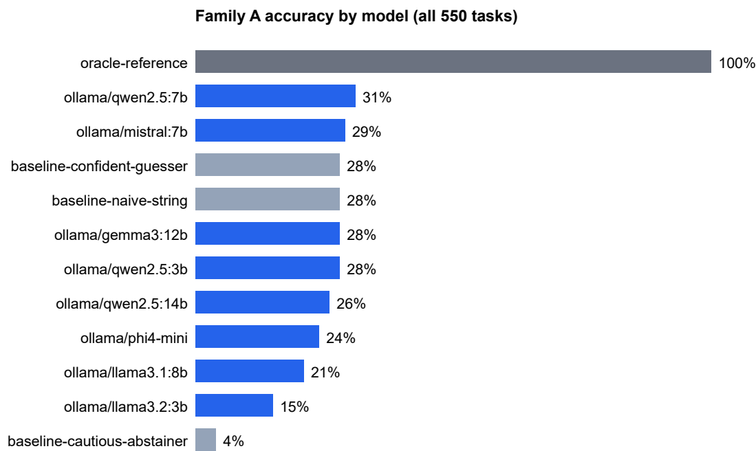
Family A accuracy by model, all 550 tasks
