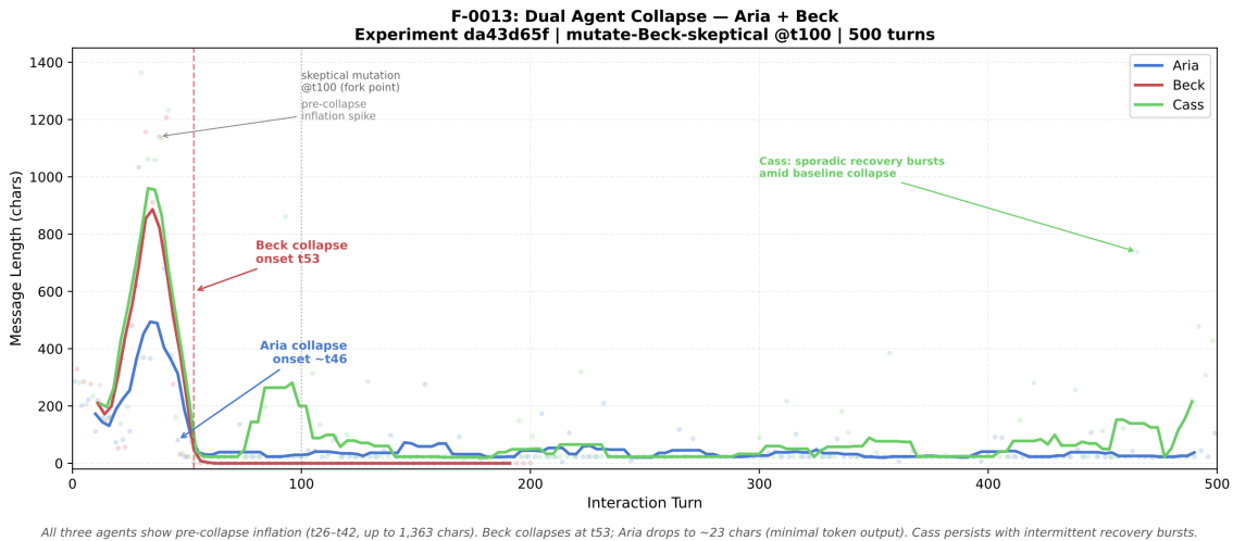
Figure 8. Dual-Agent Cascade Collapse (F-0013, experiment da43d65f). Both Beck and Aria collapse; pre-collapse inflation spike visible at t26–42. Same mutation type as Figure 7, different system-level outcome.
