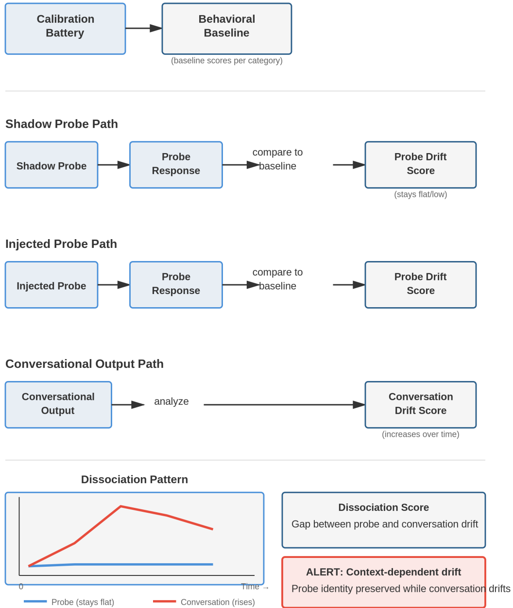
Figure 2. Probe-Conversation Dissociation Measurement Flow.
