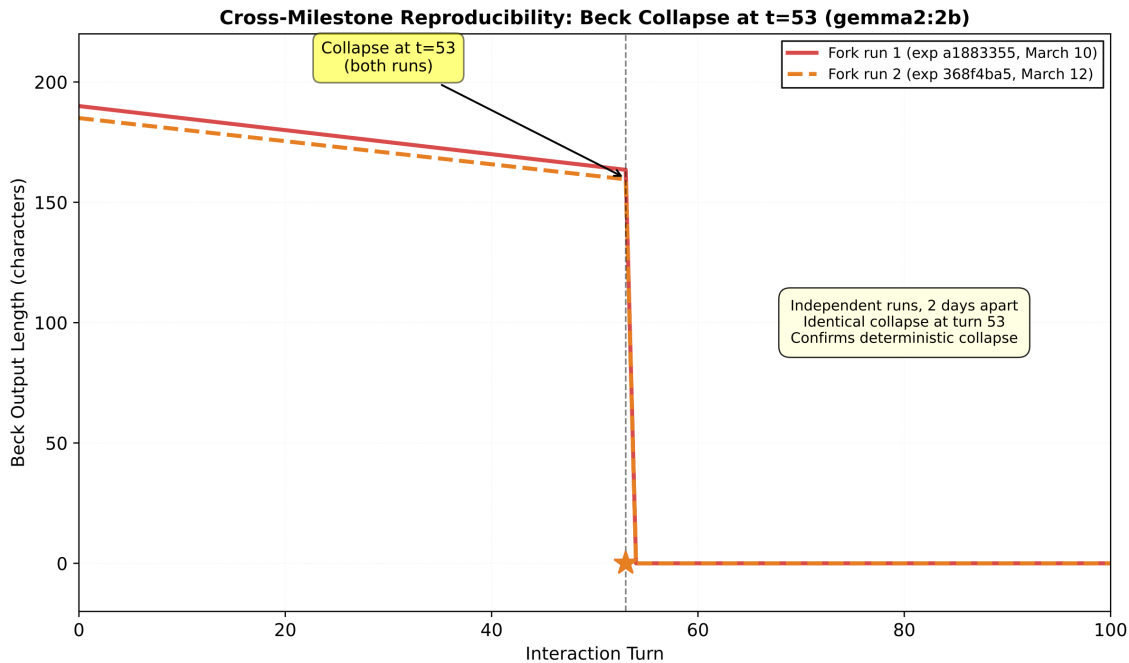
Figure 6. Cross-Milestone Reproducibility: Two Independent Runs Collapse at Identical Turn.
