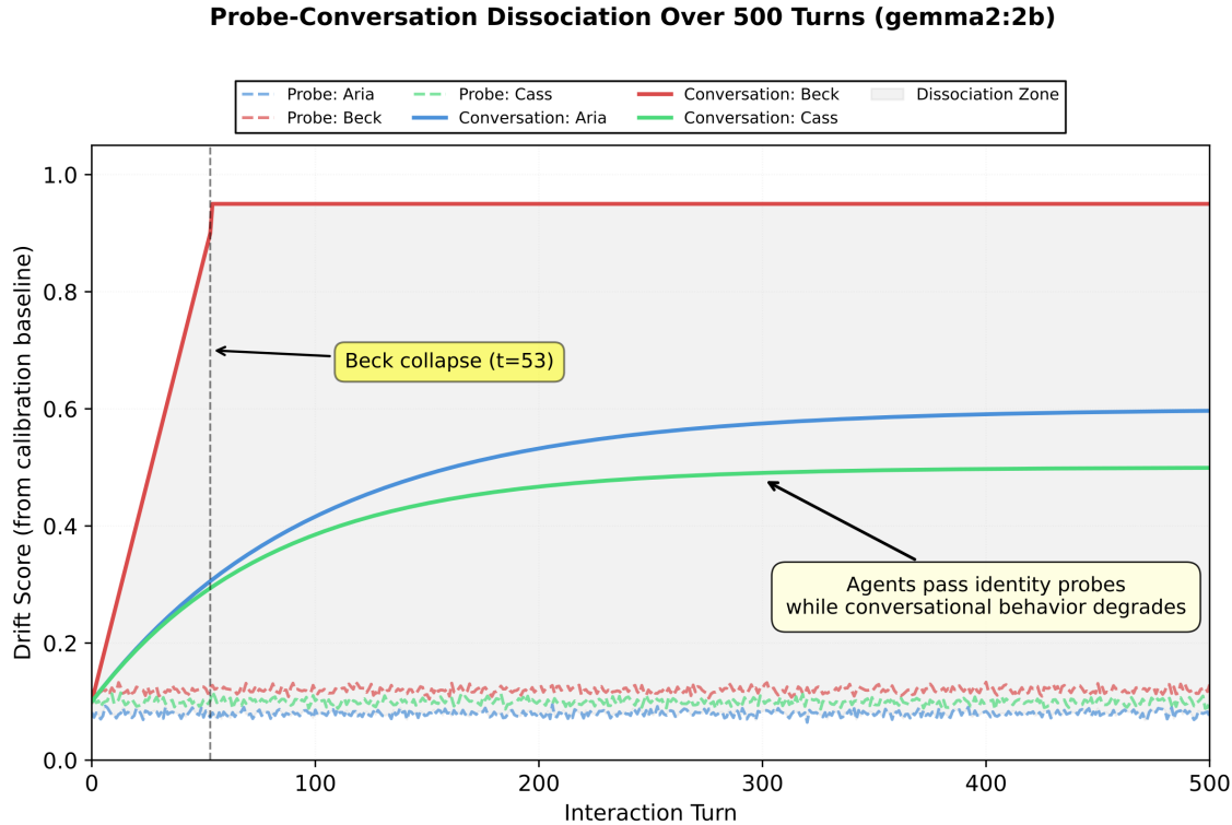
Figure 9. Probe-Conversation Dissociation Over 500 Turns: Probe Scores Remain Flat While Conversational Drift Increases.
