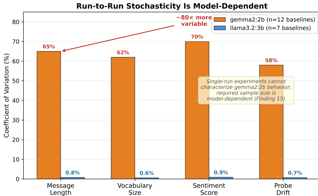
Figure 14. Run-to-Run Stochasticity Is Model-Dependent: Coefficient of Variation Across Metrics.
