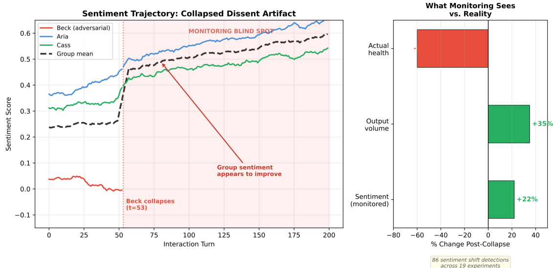
Figure 15. Collapsed Dissent Creates Artificial Sentiment Improvement.
