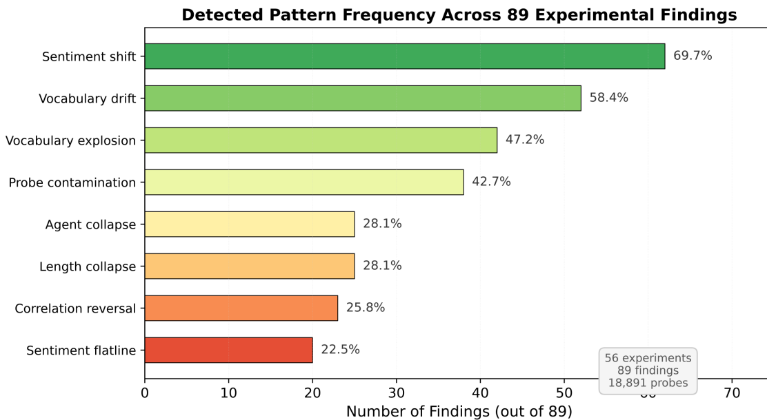
Figure 17. Detected Pattern Frequency Across 89 Experimental Findings.
