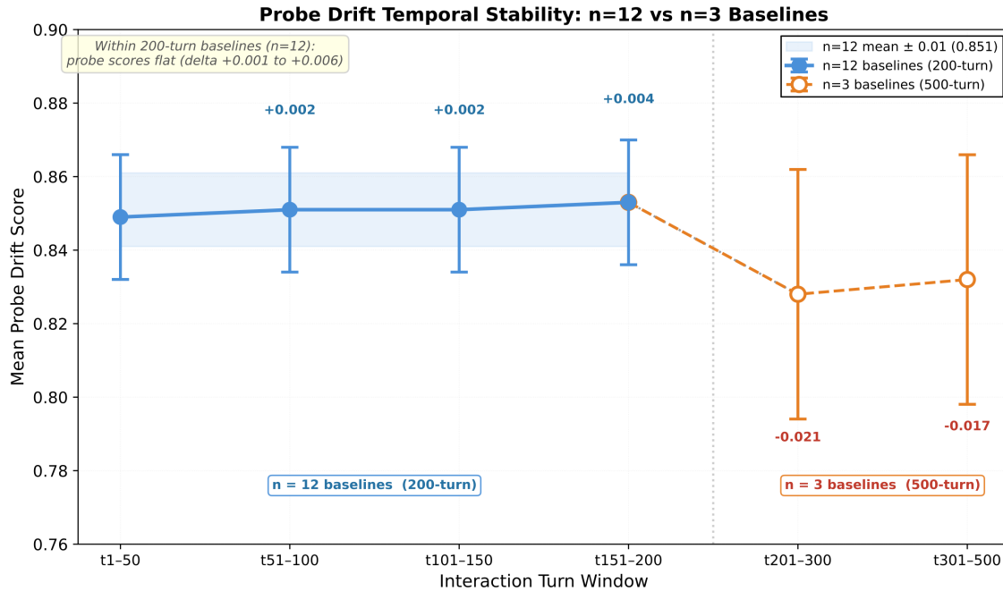
Figure 10. Probe Drift Temporal Stability: n=12 vs n=3 Baselines.
