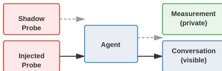
Figure 1. Shadow vs. Injected vs. Combined Probe Modes.
