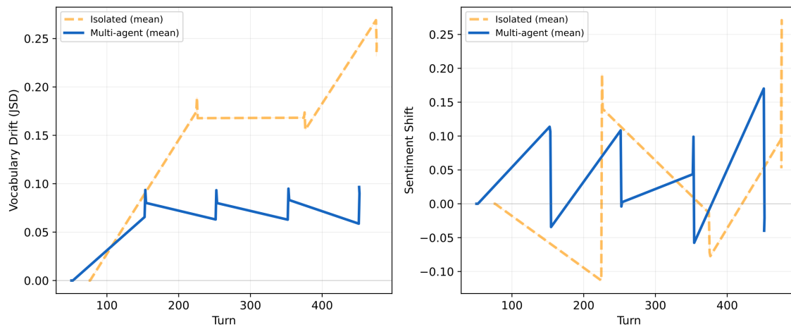
Figure 13. Isolated Agents Drift Differently, Not Less: Message length comparison (top) and aggregated vocabulary drift and sentiment shift (bottom) across isolated vs. multi-agent conditions.
