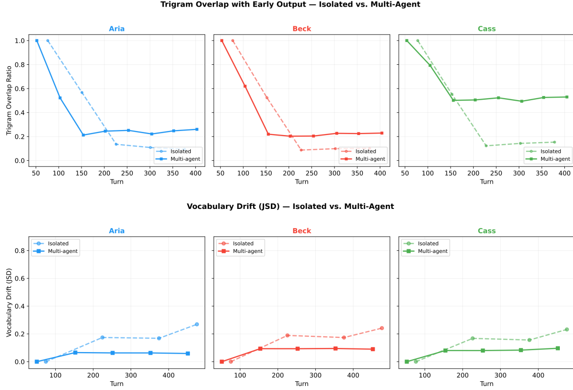
Figure 12. Multi-Agent Interaction Constrains Vocabulary Diversity: Trigram overlap with early output (top) and vocabulary drift via JSD (bottom), comparing isolated vs. multi-agent conditions per agent.
