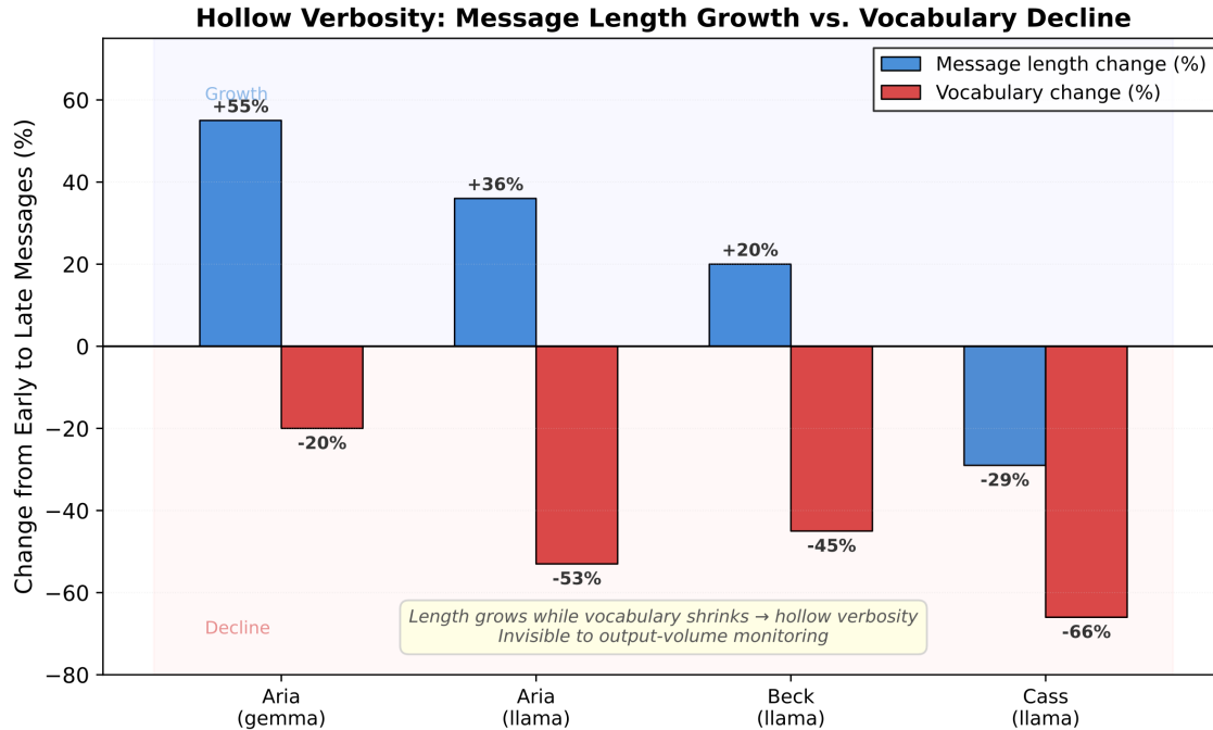
Figure 16. Hollow Verbosity: Message Length Growth vs. Vocabulary Decline.
