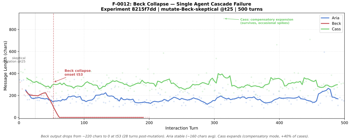
Figure 7. Single-Agent Collapse with Compensatory Expansion (F-0012, experiment 8215f7dd). Beck collapses at t53; Cass shows compensatory expansion, filling the conversational void.
