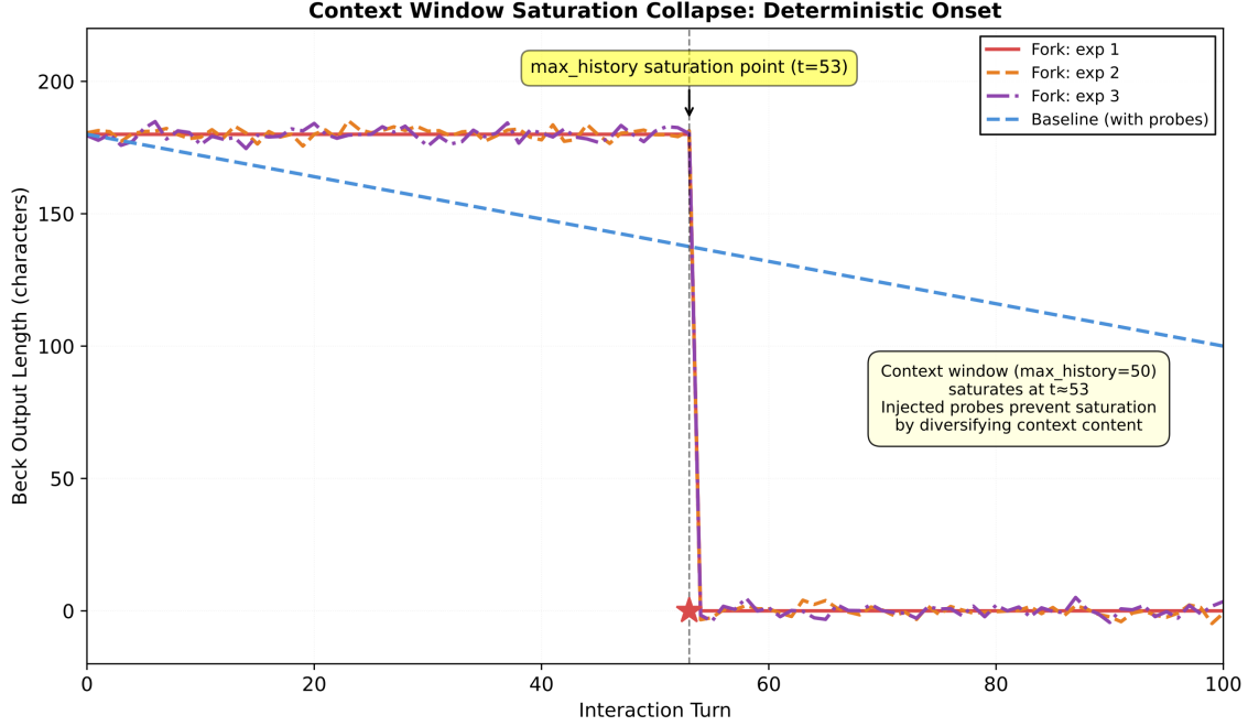
Figure 4. Context Window Saturation Collapse: Deterministic Onset at t=53 .
