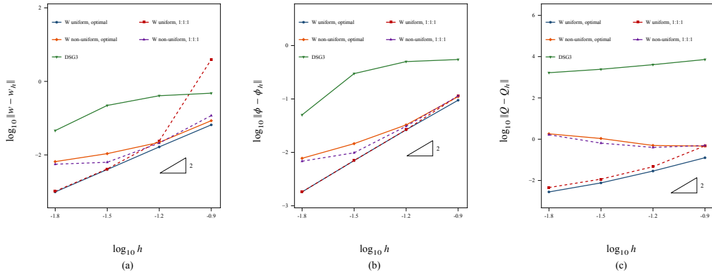
q, \varphi : tri3 FEM; w : meshfree RK. From left to right (ndiv = 64/32/16/8): n_q = n_\varphi = 4225/1089/289/81 ; n_w = 4096/1024/256/64 (optimal ratio) or n_w = n_q (1:1:1). W non-uniform: gmsh random unstructured meshes; DSG3 is displacement-based and has no independent q , so its (c) curve is the raw shear strain \|\gamma_h\| .
