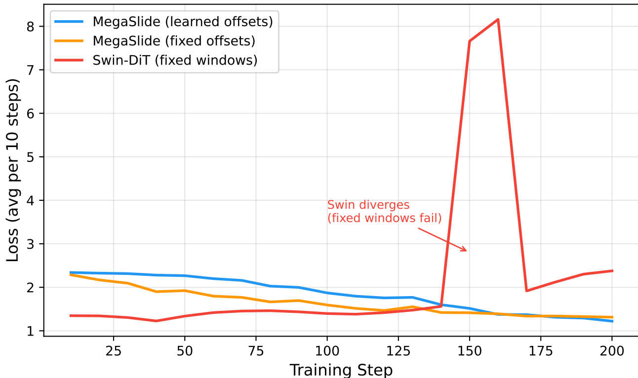
Quality Ablation: Swin Diverges on Temporal Motion Data (256 frames)
