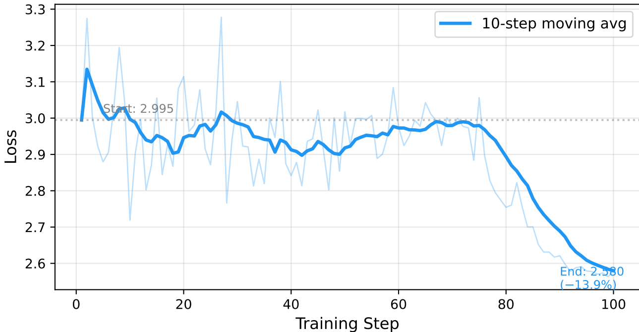
28.4B MegaSlide-DiT: Training Convergence (100 steps, 63 min)
