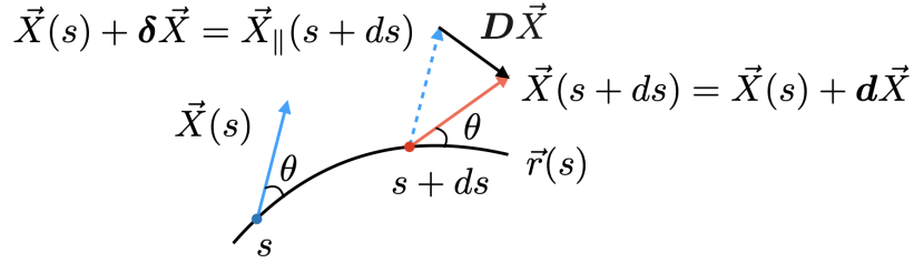
Fig. 3.17: Parallel transport of vector \vec{X} .
