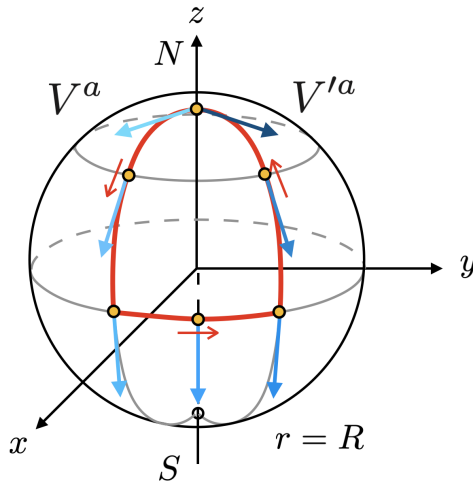
Fig. 3.20: Parallely transported a vector V^a along a closed loop (red solid line) counterclockwise on a sphere.
