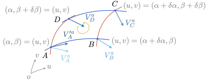
Fig. 3.19: Parallel transport of a vector V^a around a closed loop counterclockwise in a curved space.
