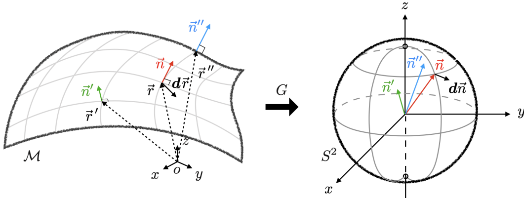
Fig. 3.21: The Gauss map G of a surface.
