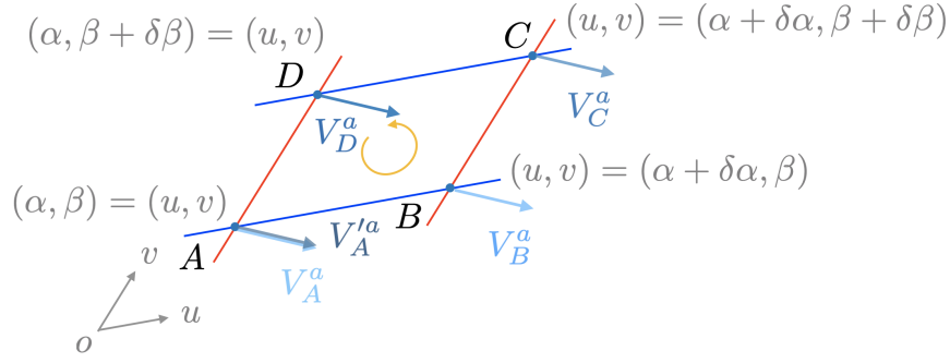
Fig. 3.18: Parallel transport of a vector V^a around a closed loop counterclockwise in a flat space.
