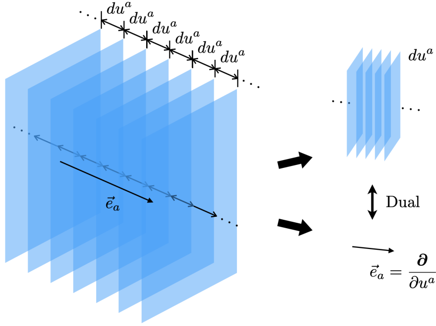
Fig. 3.13: Dual bases of the u^a -coordinate.
