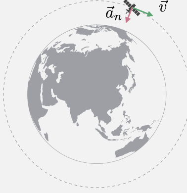
Fig. 3.15: The circular motion of a satellite.
