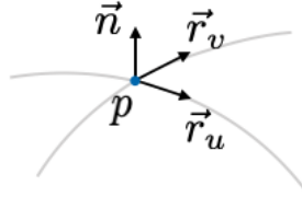
Fig. 3.14: A local frame of \mathcal{M} .
