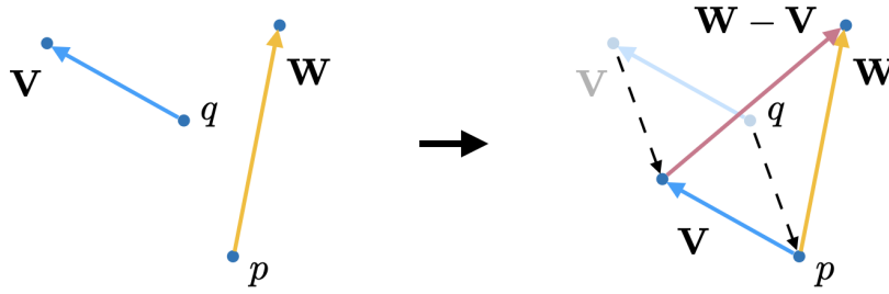
Fig. 1.3: Comparison of two vectors \mathbf{V} and \mathbf{W} at the sam point.
