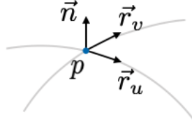
Fig. 3.14: A local frame of \mathcal{M} .
