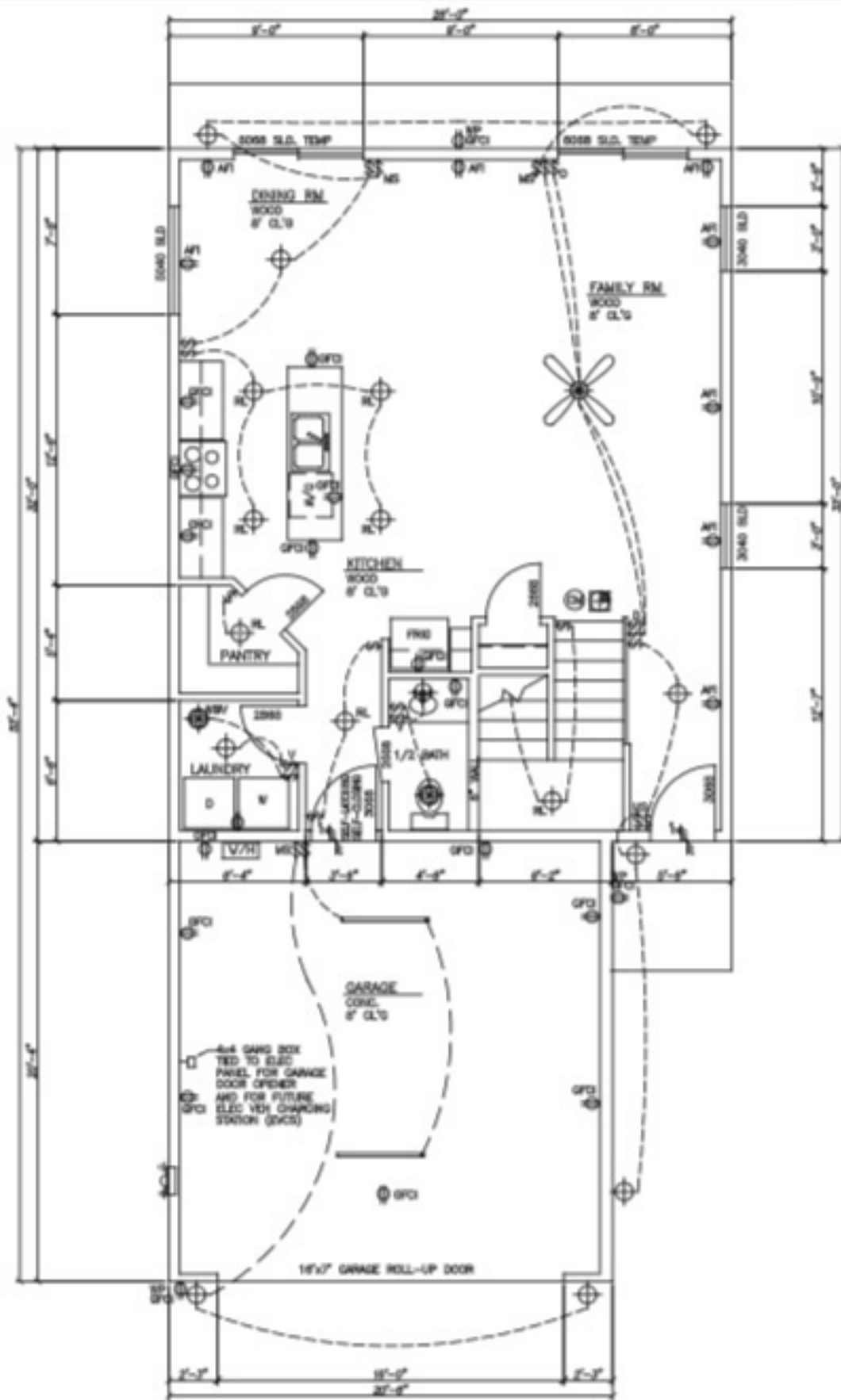
FLOOR 1 PLAN
