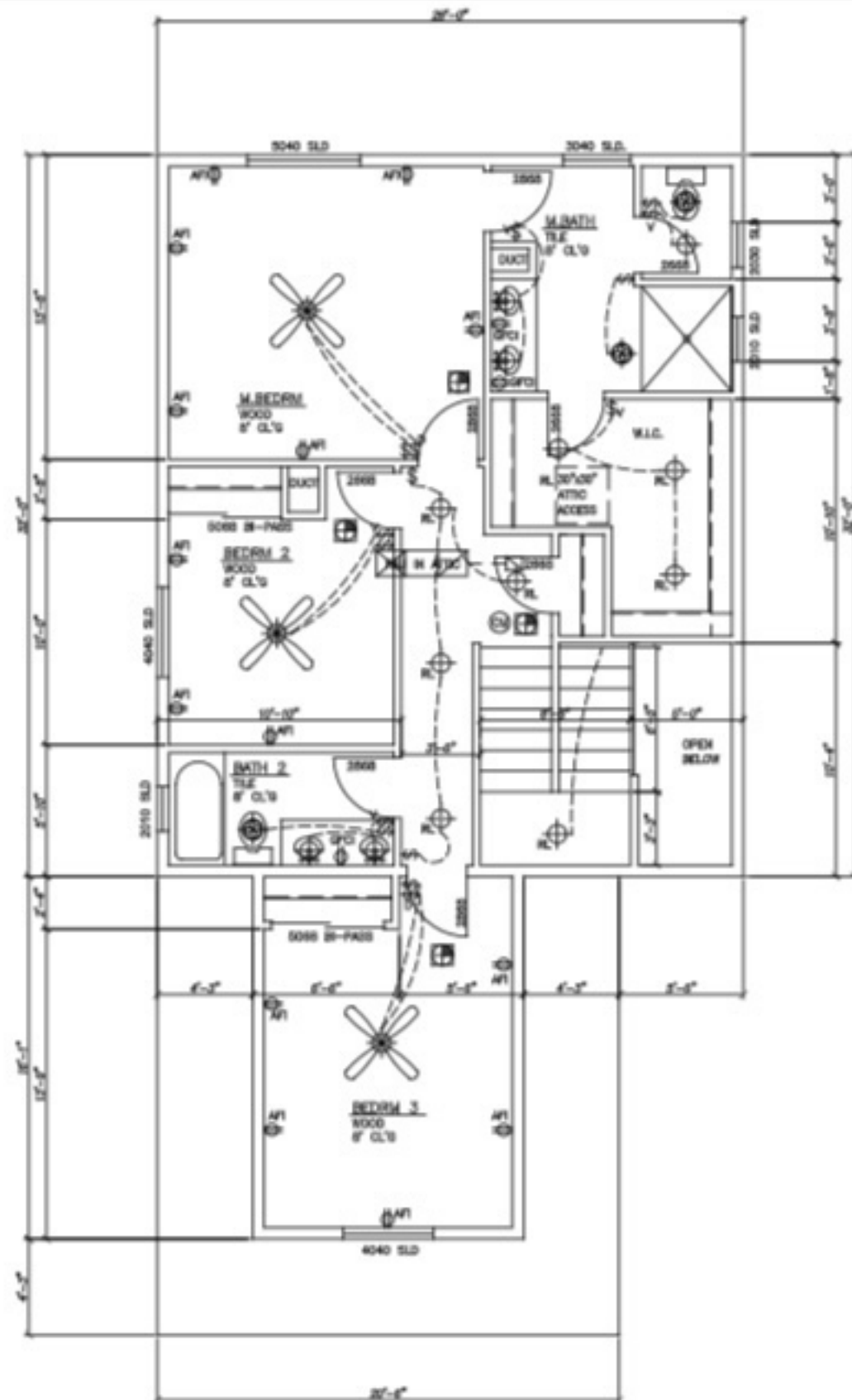
FLOOR 2 PLAN
