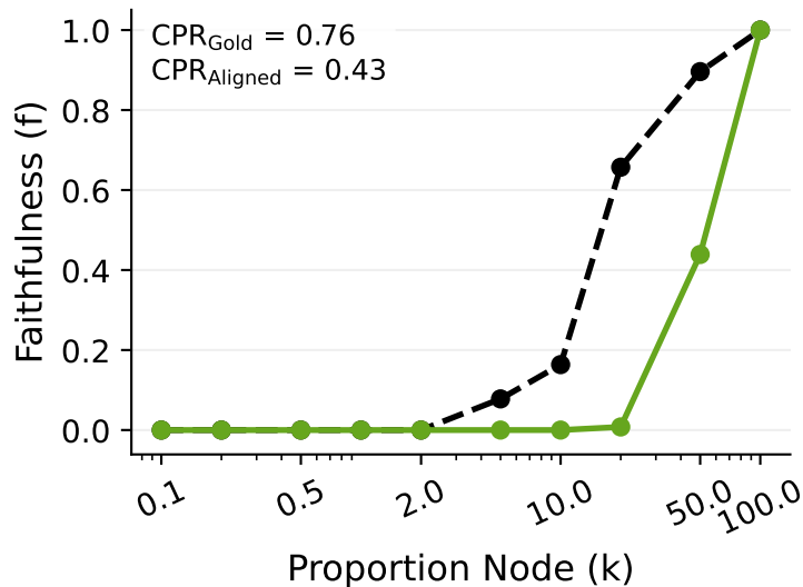
ARC-Easy
