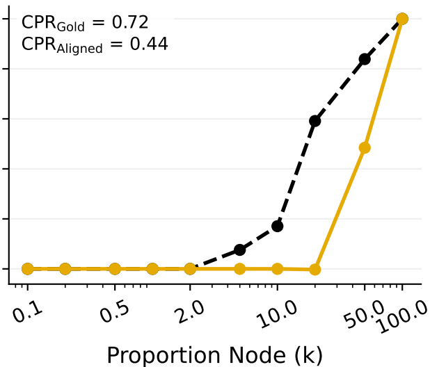
ARC-Challenge
