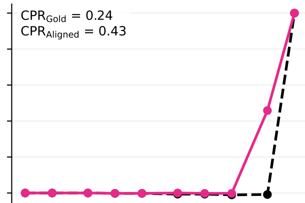
Subtraction
