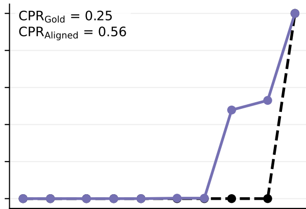
Addition
