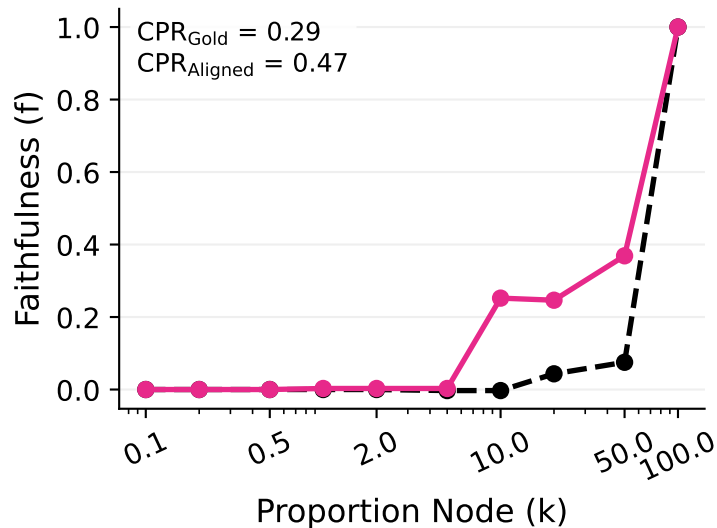
Subtraction
