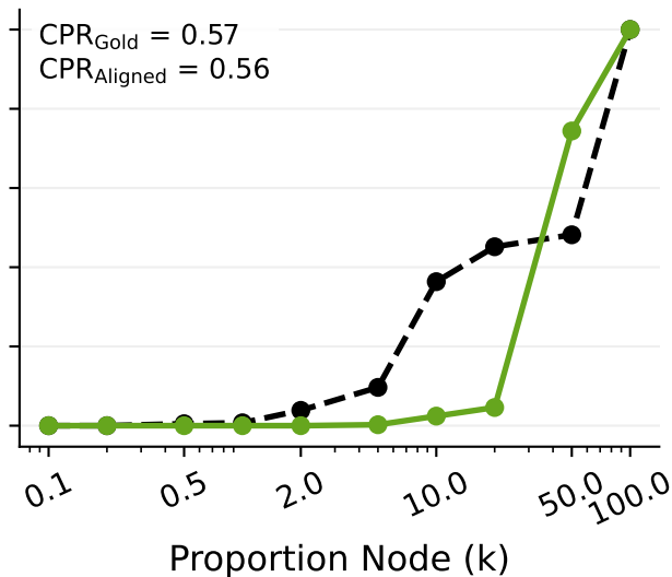
ARC-Easy
