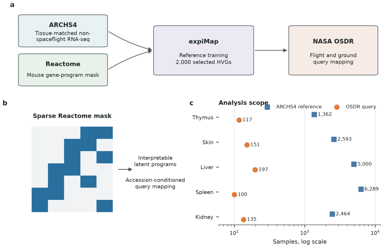
Figure 1. Reference-guided workflow, constrained architecture, and analysis scope. a , Tissue-matched non-spaceflight ARCHS4 profiles and current mouse Reactome memberships independently define each reference model; NASA OSDR flight and ground profiles are then mapped as accession-conditioned queries. b , The sparse architecture connects measured genes to annotated latent programs. c , Reference and primary-query sample counts for the four positive-result tissues and secondary kidney model. Spleen shows the 100 samples retained for its primary effect after excluding OSD-288.
